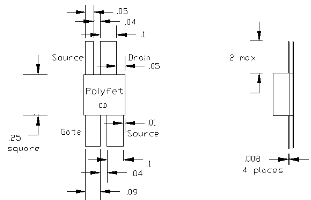
PACKAGE DIMENSIONS IN INCHES
