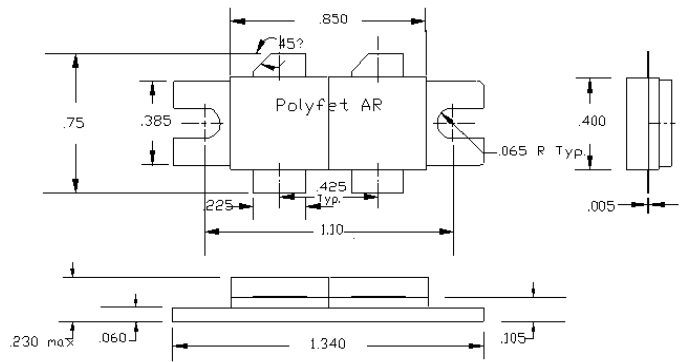
PACKAGE DIMENSIONS IN INCHES
