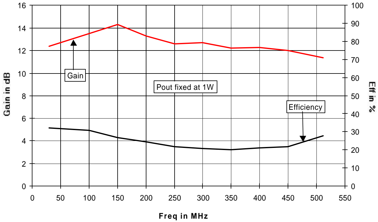
TB197 L8821P Gain/Eff. vs Freq.; Vds=12.5Vdc Idq=0.2A
